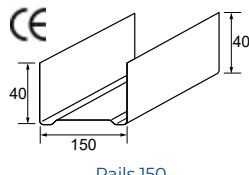
Rails 150
