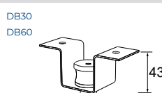
Raccord fourrure 17-55
