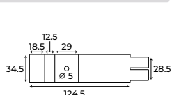
Anti-soulèvement
