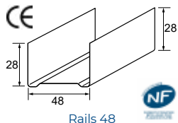
Rails 48
