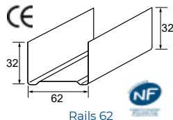
Rails 62
