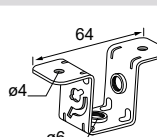
Attache Omega
