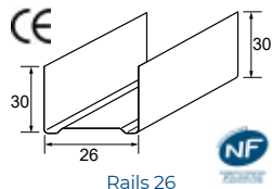
Rails 26
