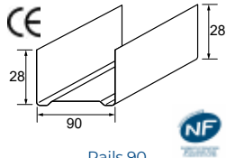
Rails 90
