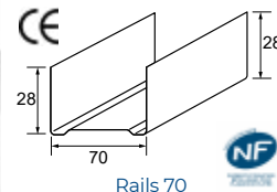
Rails 70
