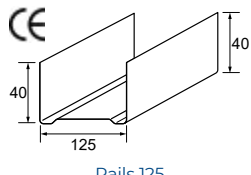
Rails 125
