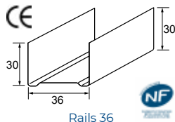
Rails 36
