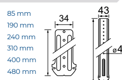
Suspentes fourrure 18-45
