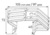
Attache de suspension
